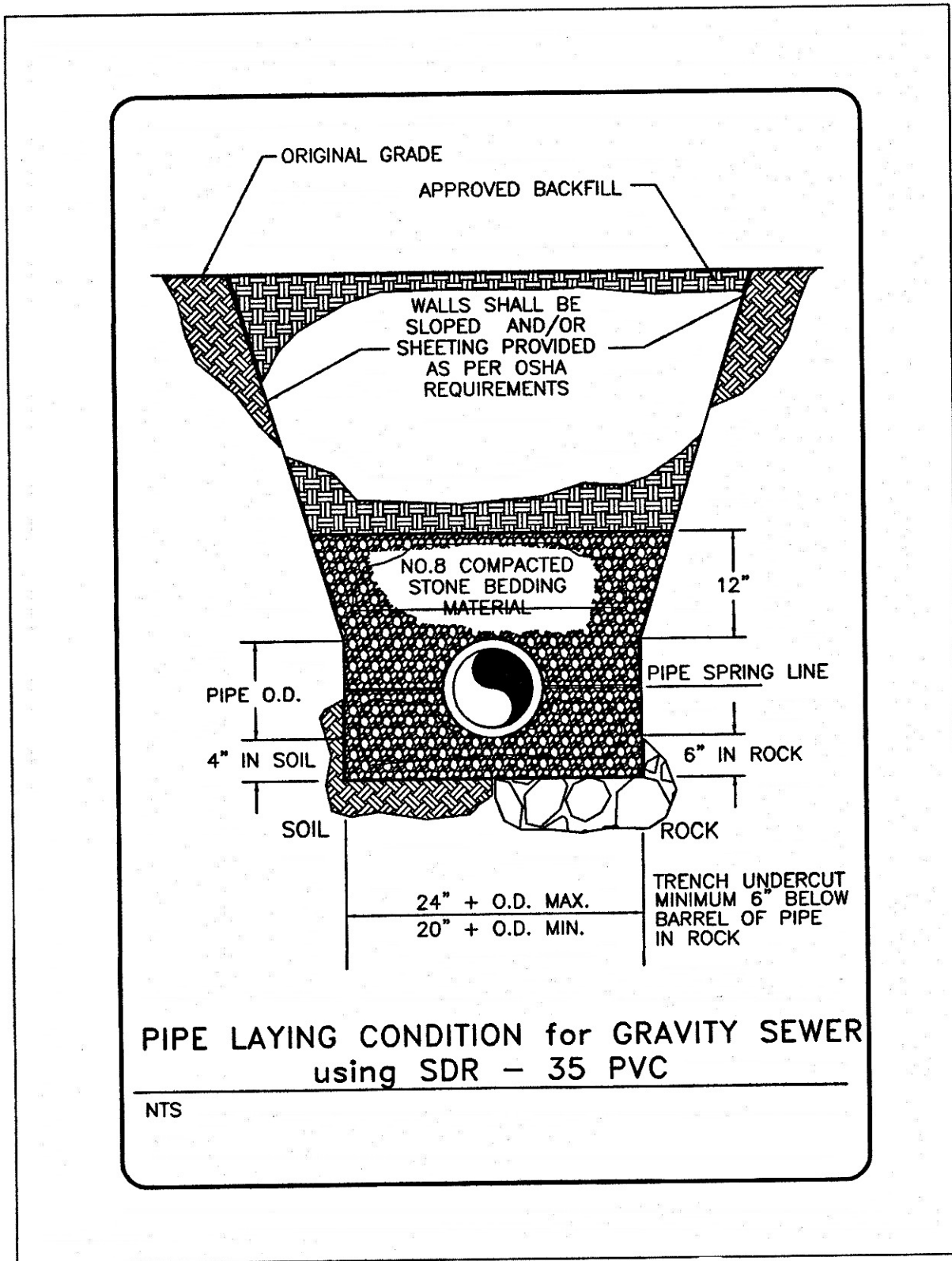
Figure 7. Pipe Laying Condition for Gravity Sewer Using SDR-35 PVC
